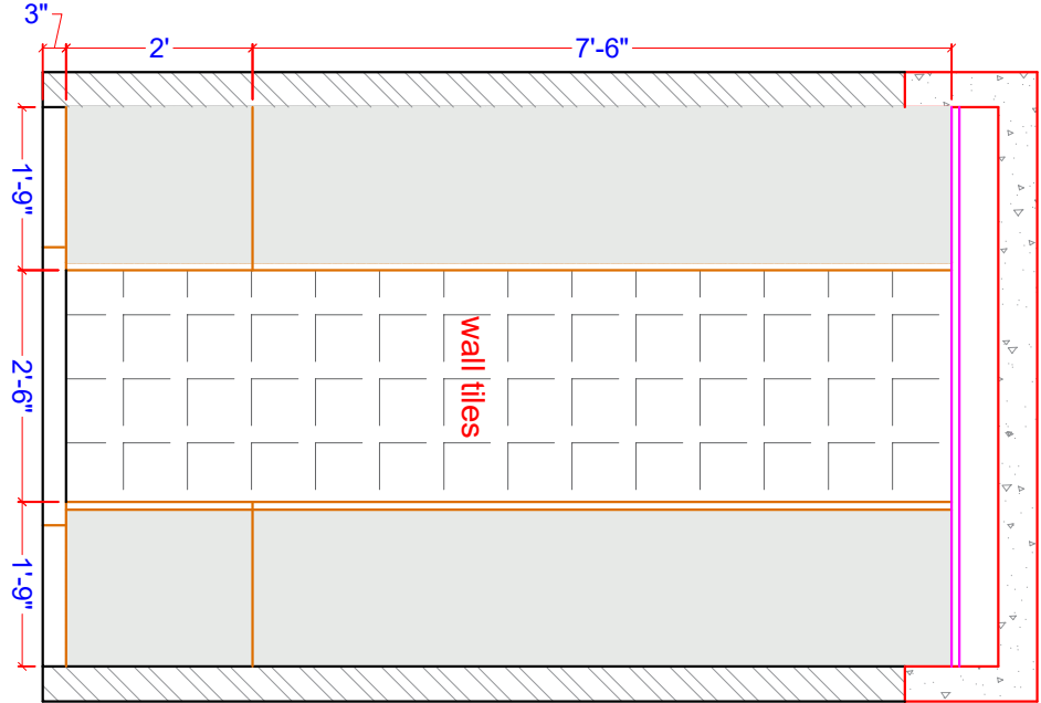
WALL ELEVATION - B
