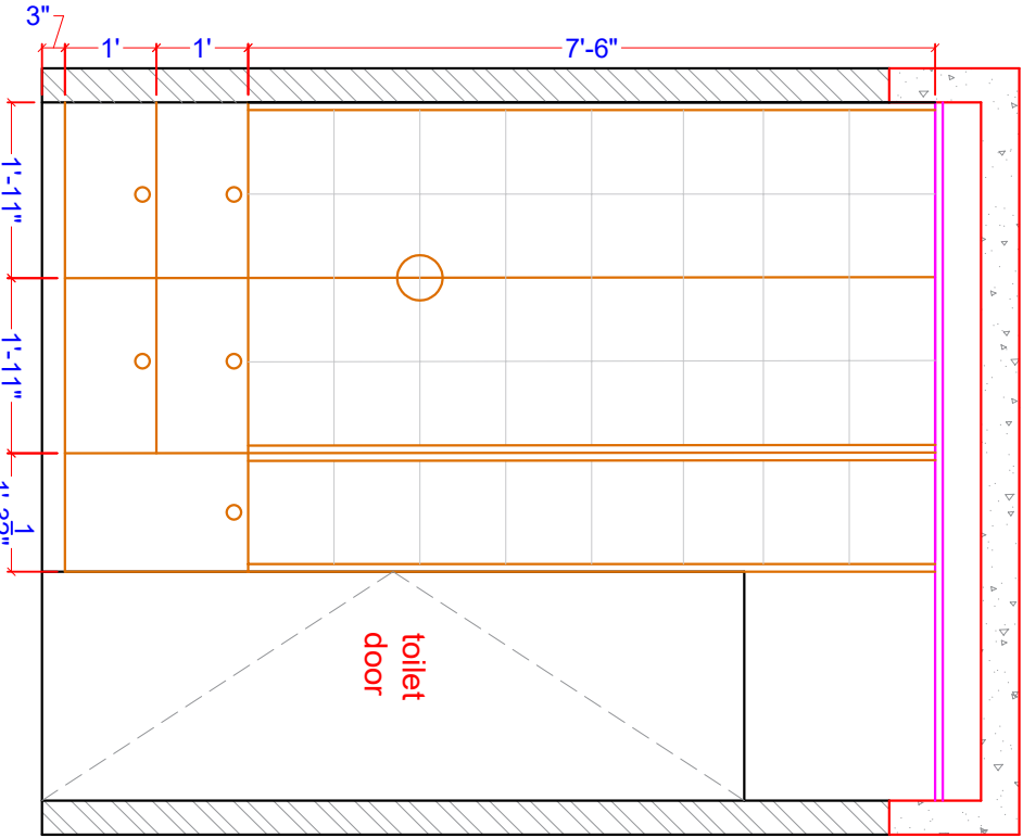
WALL ELEVATION - C
