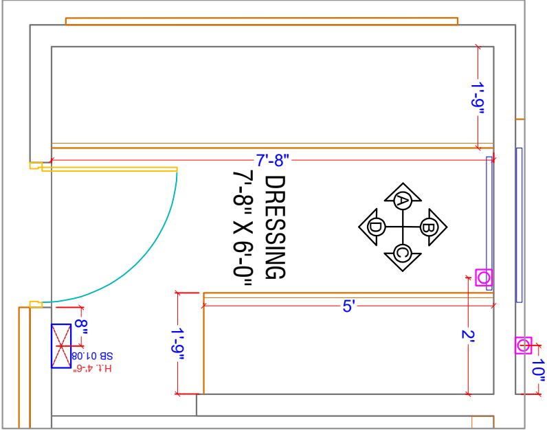
KID'S WALKING WARDROBE PLAN
