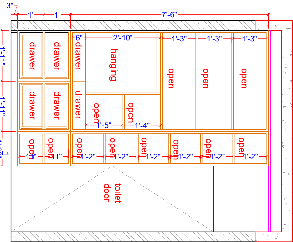
WALL - C internal details
