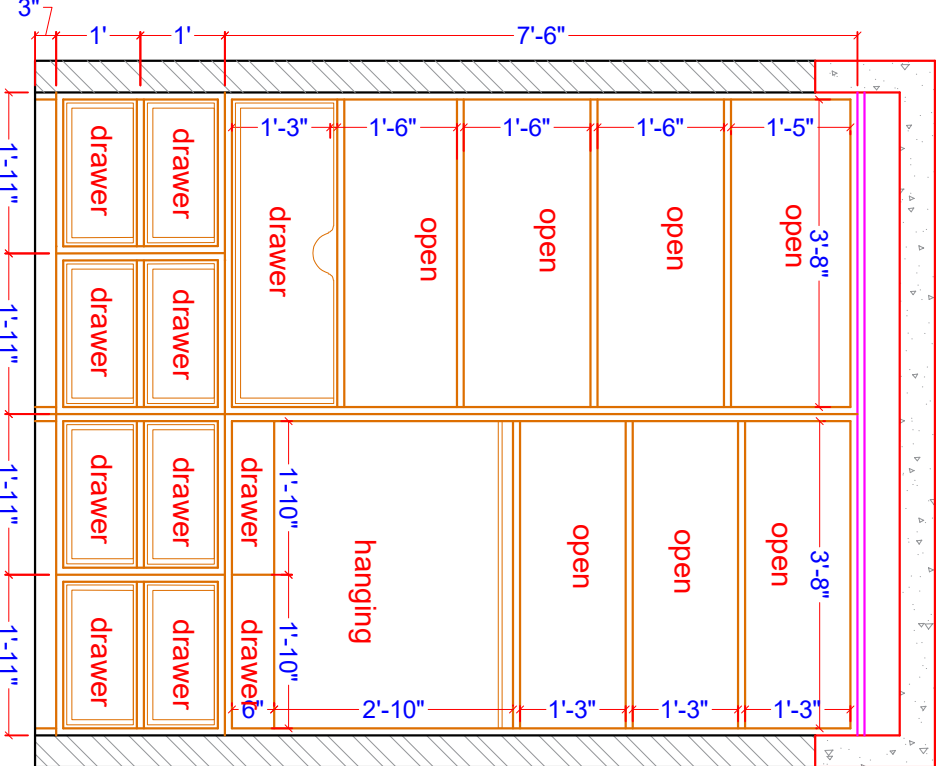
WALL ELEVATION - A
