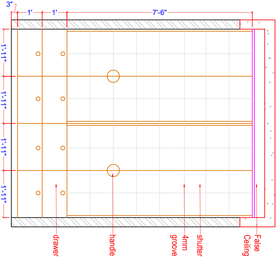
WALL ELEVATION - A
